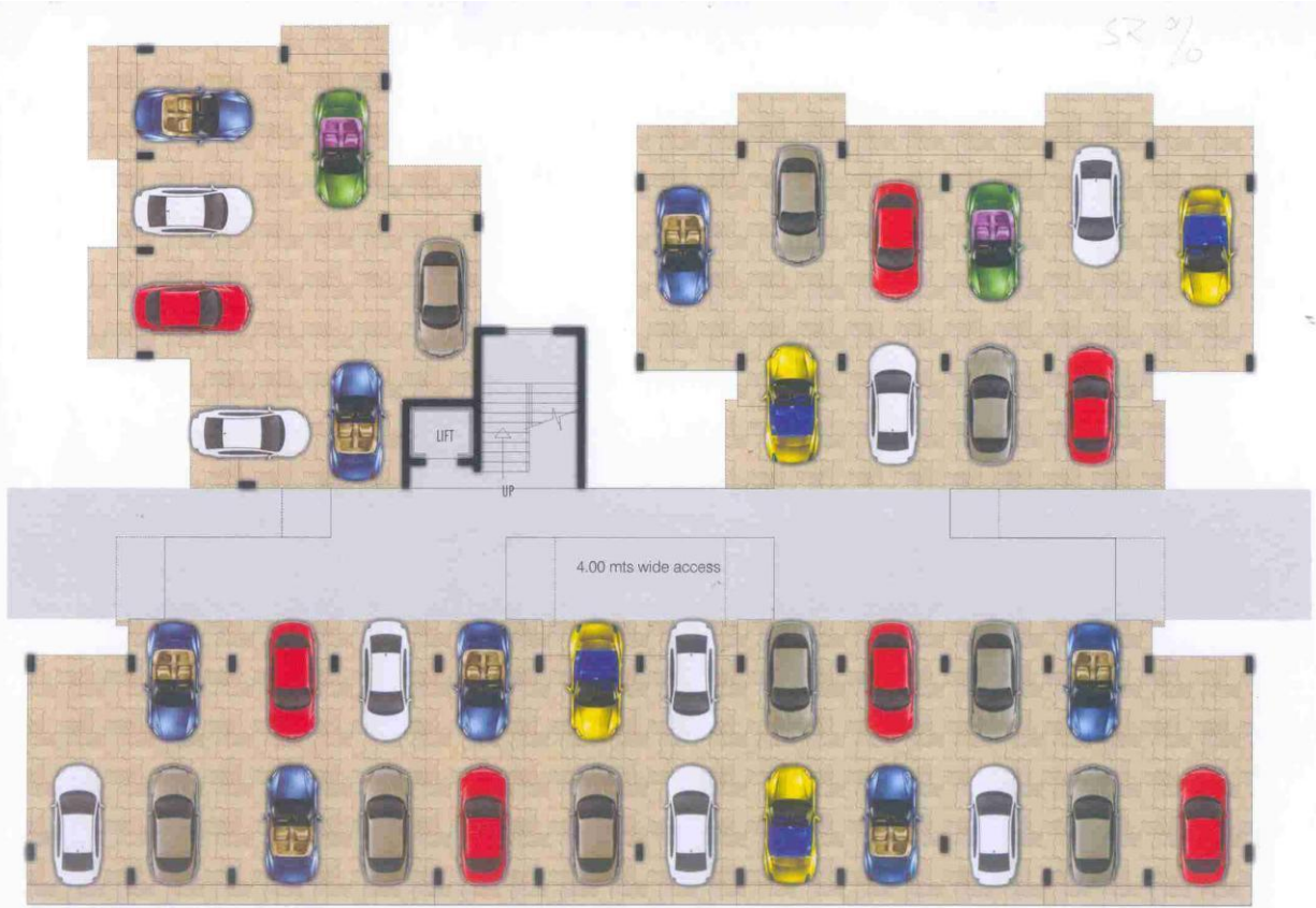
BUILDING B - Stilt floor plan
